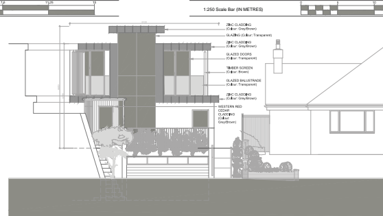
HOUSE B, Southern Elevation (Front) Scale 1:100
