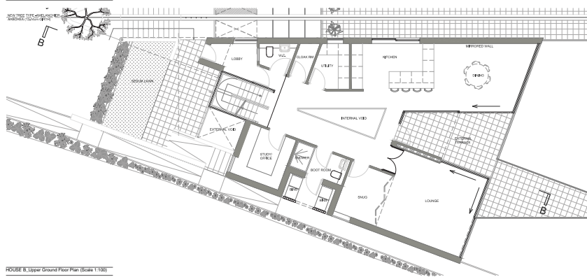
HOUSE B, Upper Ground Floor Plan (Scale 1:100)
