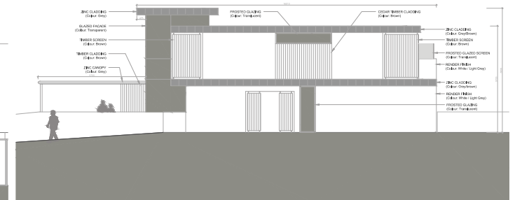
HOUSE B, Eastern Elevation (Front) Scale 1:100
