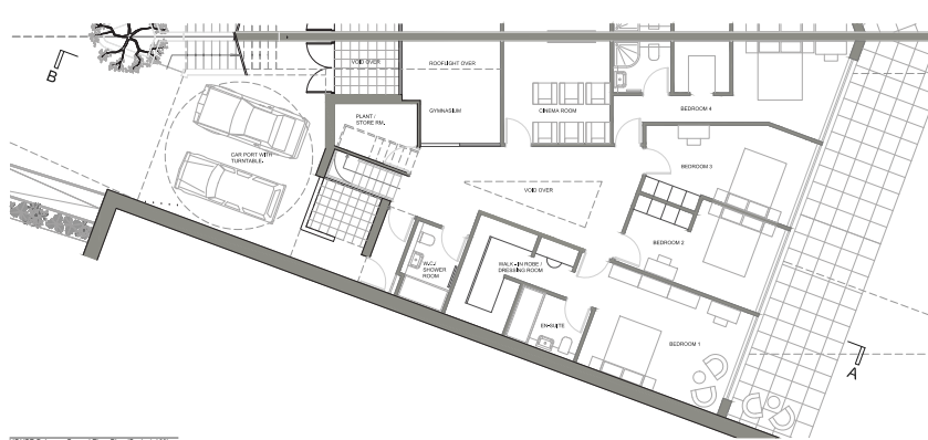
HOUSE B, Lower Ground Floor Plan (Scale 1:100)
