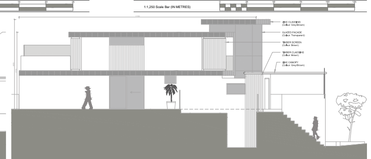
HOUSE B, Western Elevation (Side 1) Scale 1:100
