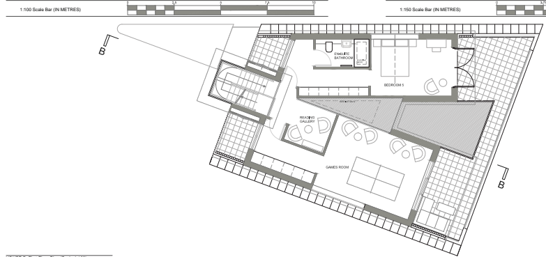
HOUSE B, First Floor Plan (Scale 1:100)
