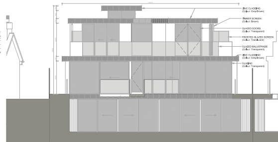
HOUSE B, Northern Elevation (Rear) Scale 1:100
